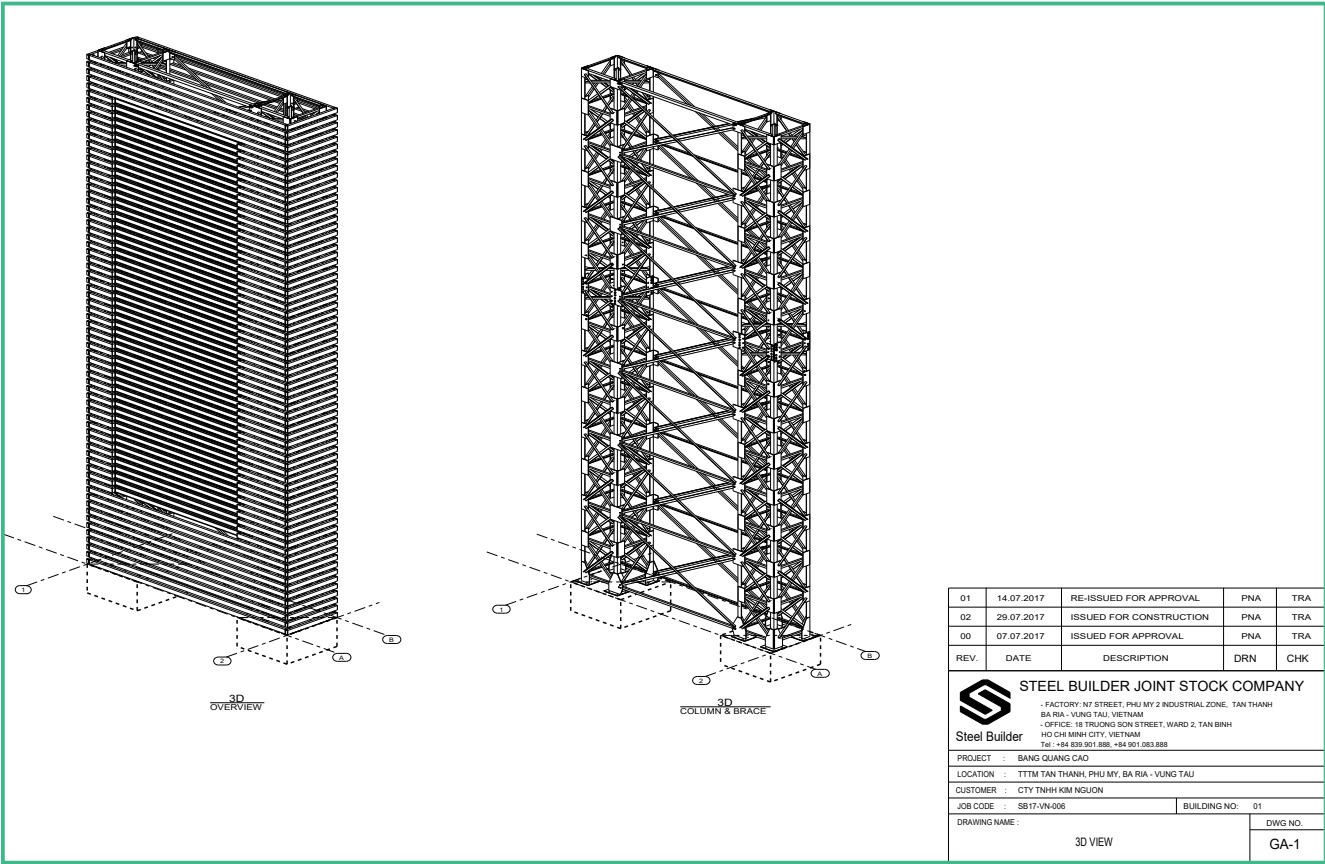
BILLBOARD STRUCTURE
